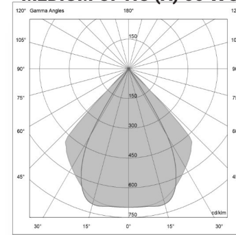
MEDIUM OPTIC (A) 60°X 86°
