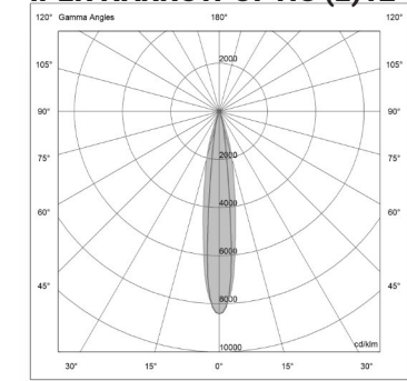
IPER NARROW OPTIC (E) 12°X 18°
