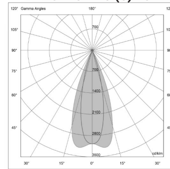
NARROW OPTIC (C) 25°X 40°
